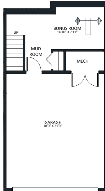
LEVEL 1 - 216 SQ. FT.
