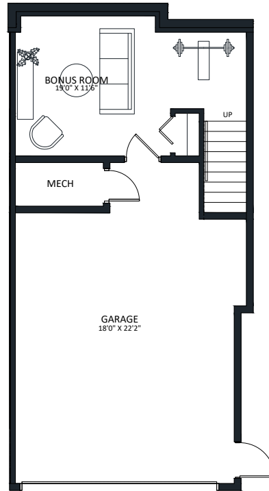
LEVEL 1 - 273 SQ. FT.
