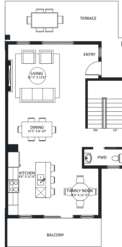
LEVEL 2 - 674 SQ. FT.
