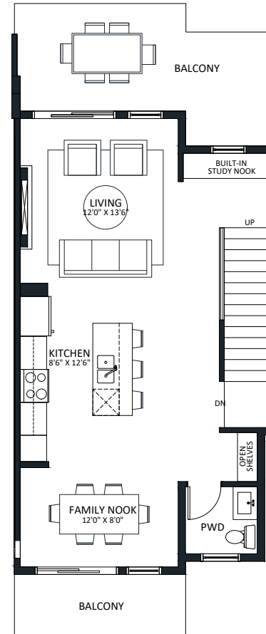
LEVEL 2 - 600 SQ. FT.
